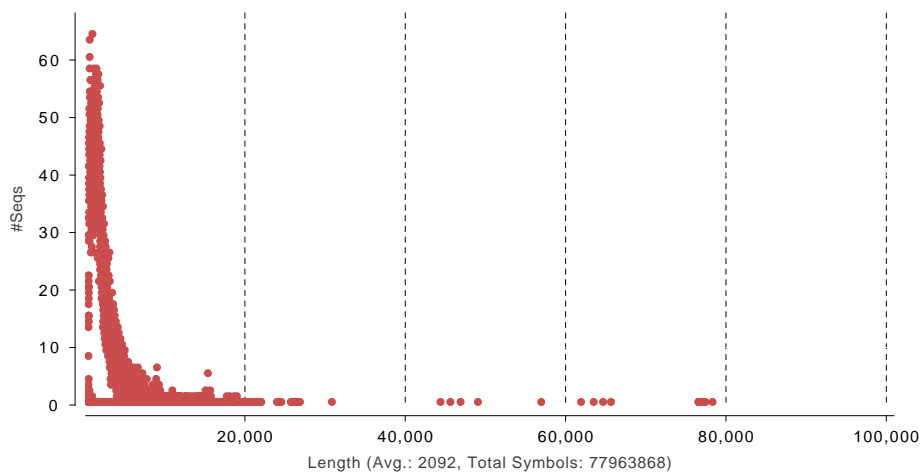
Figure: Distribution of the sequence length
