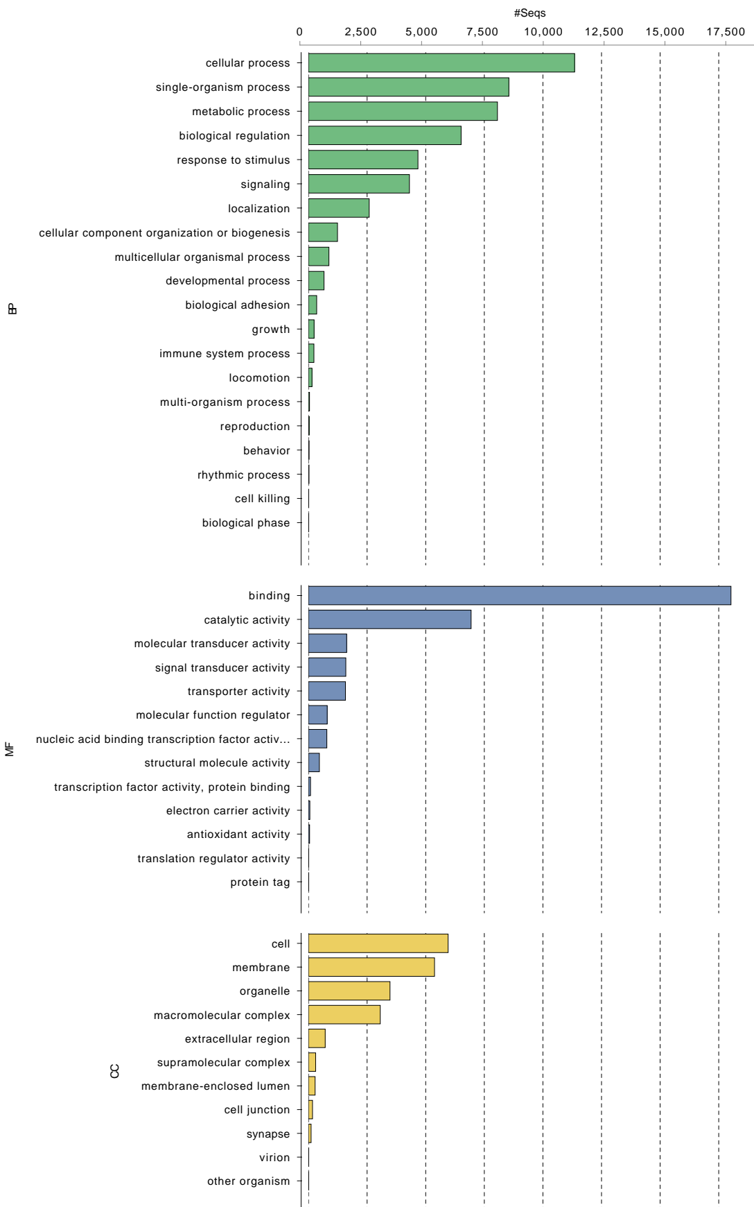
Figure: GO Distribution in Level 2 (Top 50)
